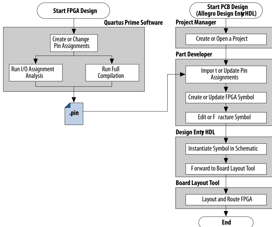
Figure 34. Design Flow with the Cadence Allegro Design Entry HDL Software
