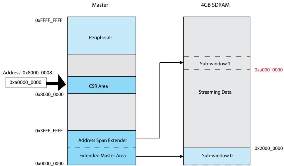
Figure 127. Memory mapping for Address Span Extender
