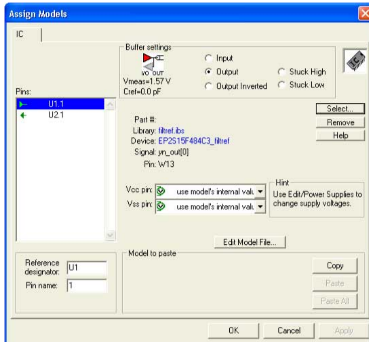
Figure 16. LineSim Assign Model Dialog Box
