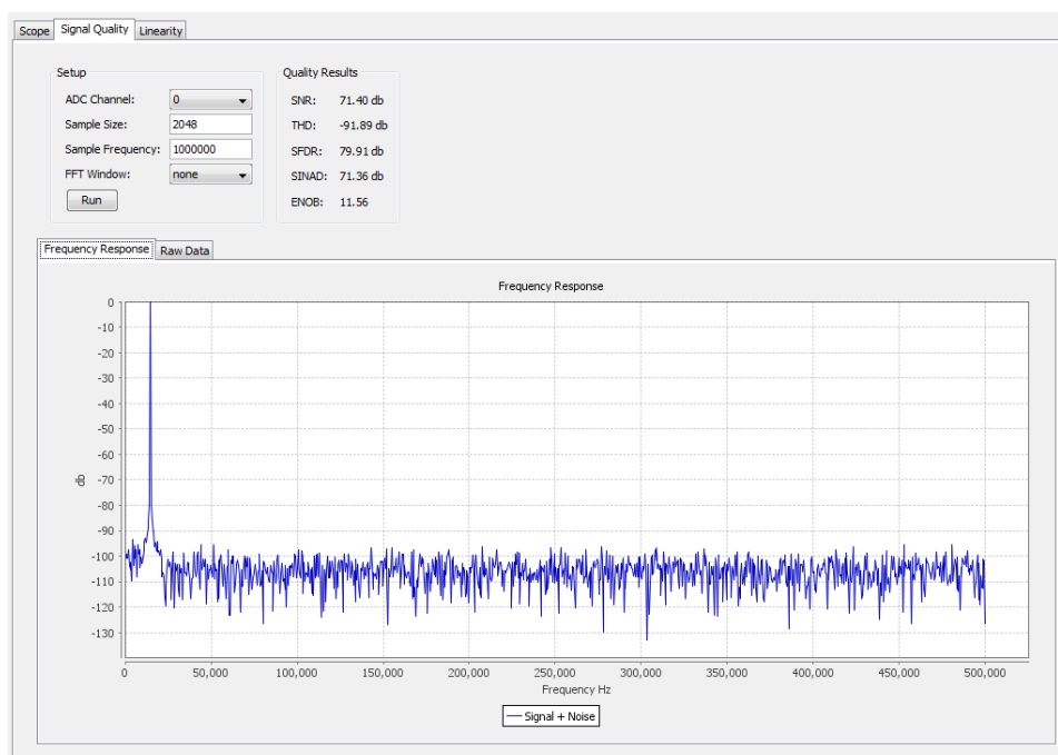
Figure 15. Signal Quality Panel
