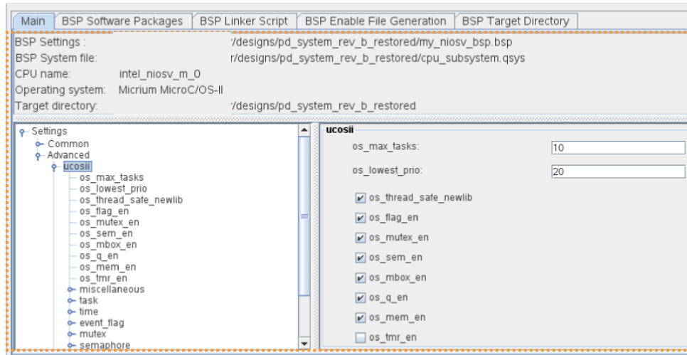
Figure 123. BSP Editor Main Tab
