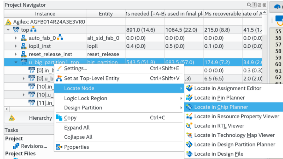
Figure 94. Locate in Chip Planner Command from Project Navigator
